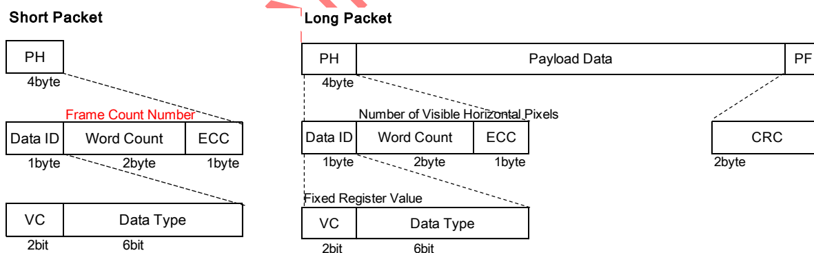
Fig. 23 Short Packet & Long Packet
