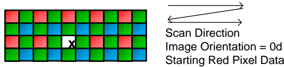
Fig. 35 Single defect
