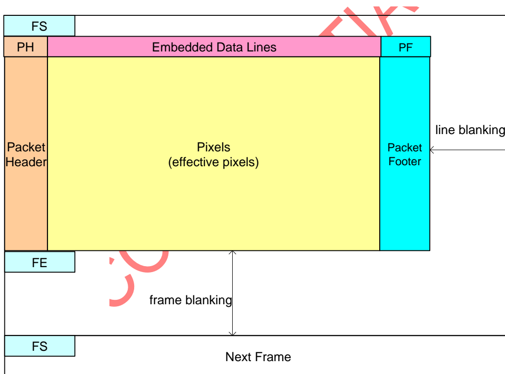
Fig. 20 Frame Structure for Serial signal output
