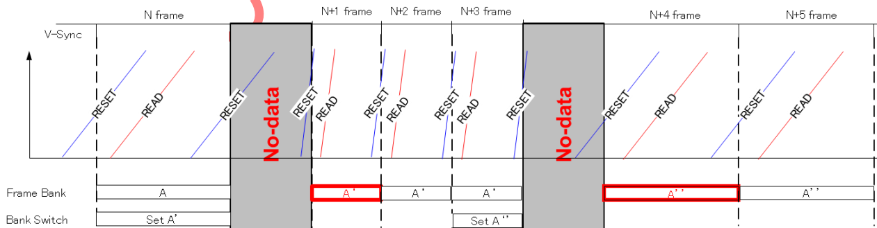
Fig. 19 Function Example for Frame Bank
